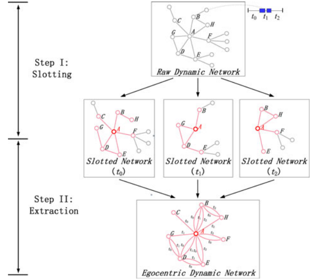
Fig. 2. An example of the egocentric dynamic network generation. The raw dynamic network is first sliced into three time slots t_0, t_1 and t_2 . Egocentric graphs are then extracted and combined. The focus node A is highlighted in red; the adjacent nodes to A and their edges are drawn in pink. The edge label identifies the corresponding time slot.
