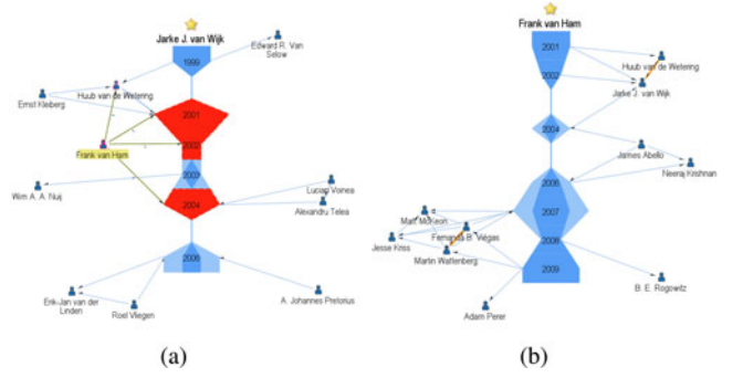
Fig. 8. Egocentric network navigation in the InfoVis co-authorship network: (a) the network central to Van Wijk, the node for Van Ham is hovered; (b) switch to the network central to Van Ham by double-clicking the node.
